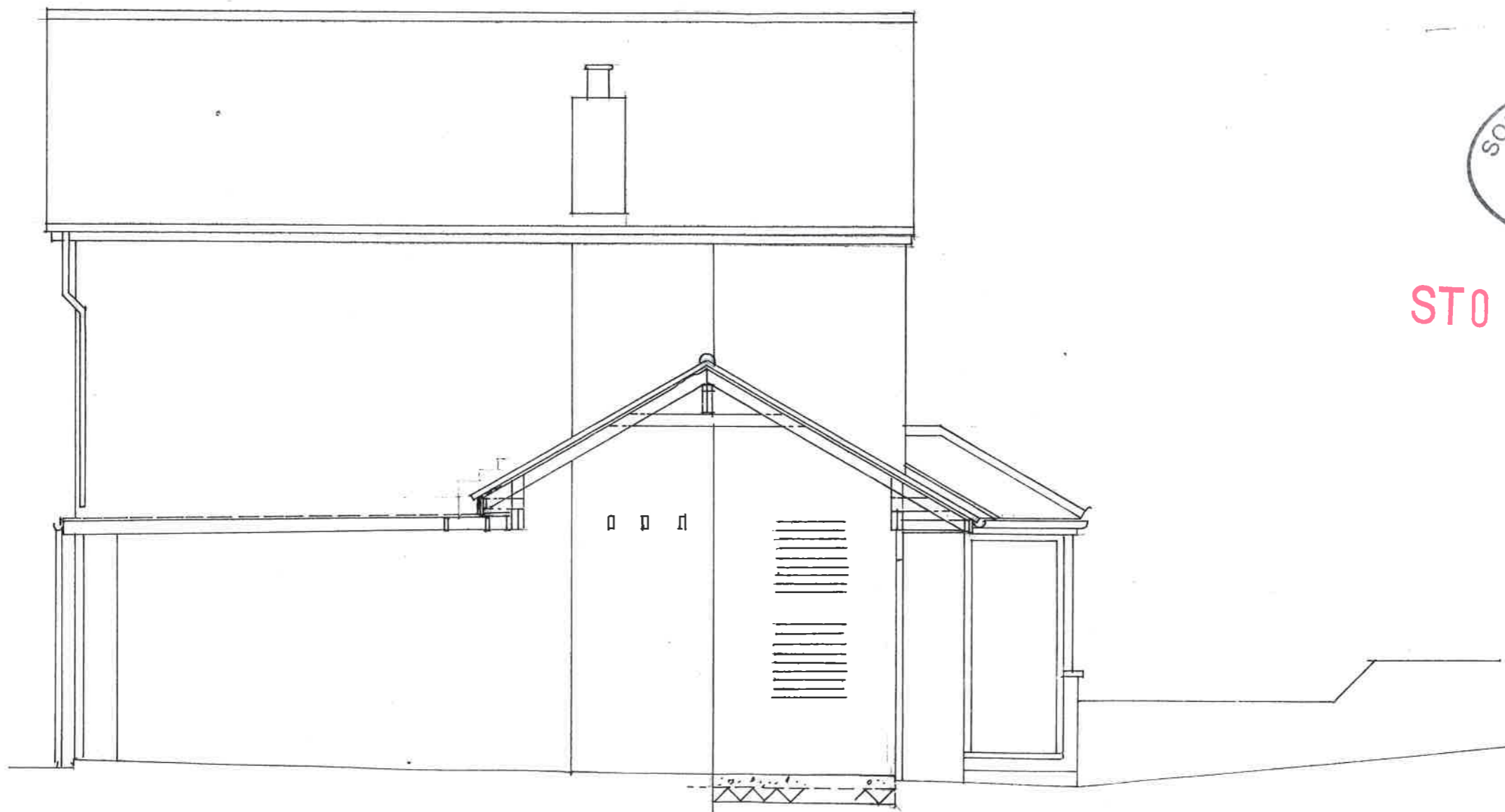
SECTION B-B
